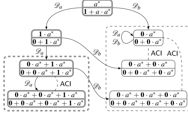
(a) norm is identity function
