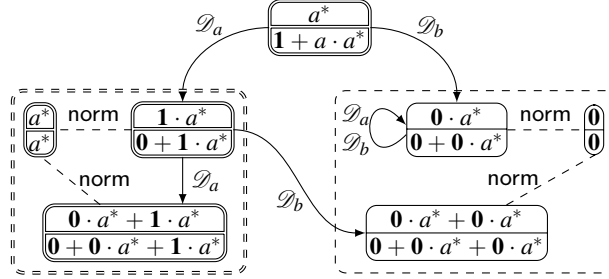
(b) norm unfolds \mathbf{0} + r = r , \mathbf{0} \cdot r = \mathbf{0} and \mathbf{1} \cdot r = r
